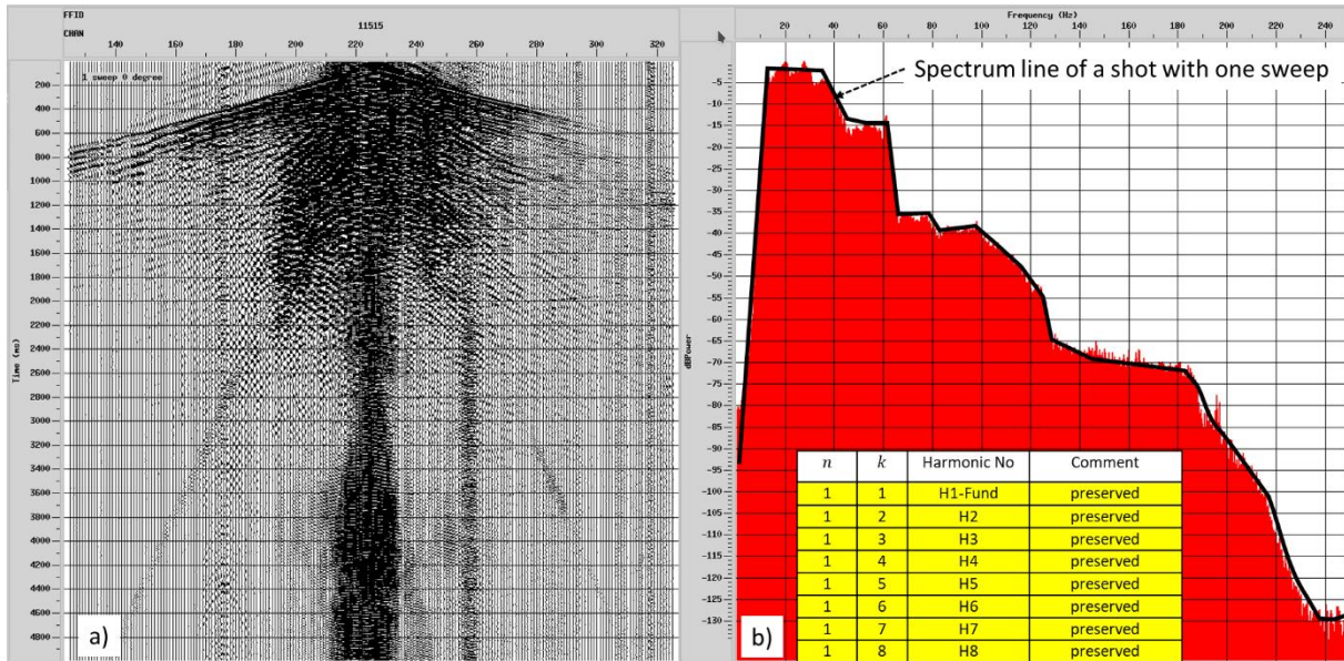
Figure 10. a) View of a 1-sweep shot with an initial phase angle of 0 degrees, b) The power spectrum of this shot
