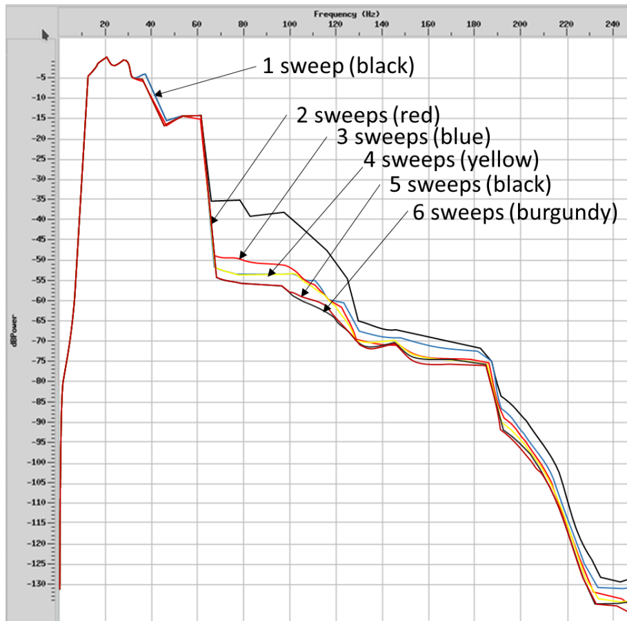
Figure 36. Graphic for harmonics elimination by sweep number
