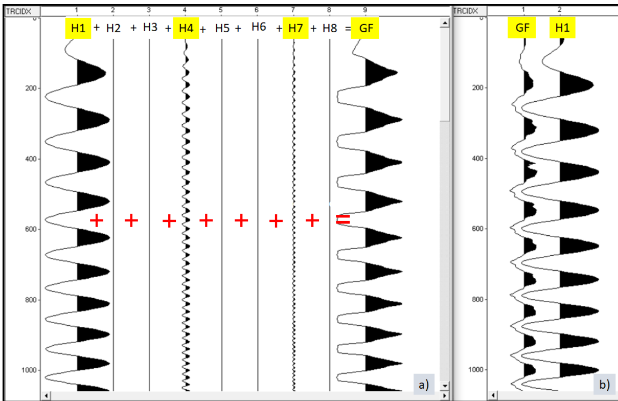
Figure 16. a) the part of synthetic fundamental sweep (H1), its harmonics (H4, H7), and GF signal, b) the part of real fundamental sweep
