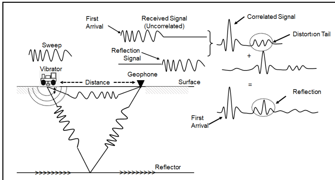
Figure 2. Schematic presentation of the vibratory surface source technique (revised from Seriff & Kim, 1970)
