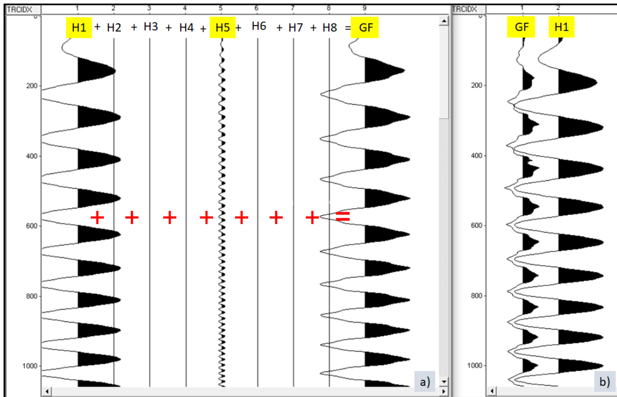
Figure 21. a) the part of synthetic fundamental sweep (H1), its harmonics (H5), and GF signal, b) the part of real fundamental sweep (H1)
