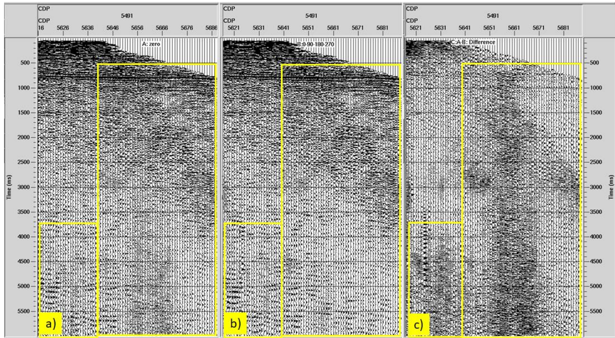
Figure 37. a) View of a 4-sweep stack with an initial phase angle of 0 degree, b) View of a 4 sweeps stack with the initial phase angles of 0, 90, 180 and 270 degrees, c) Difference between Fig. 37(a) and Fig. 37(b)
