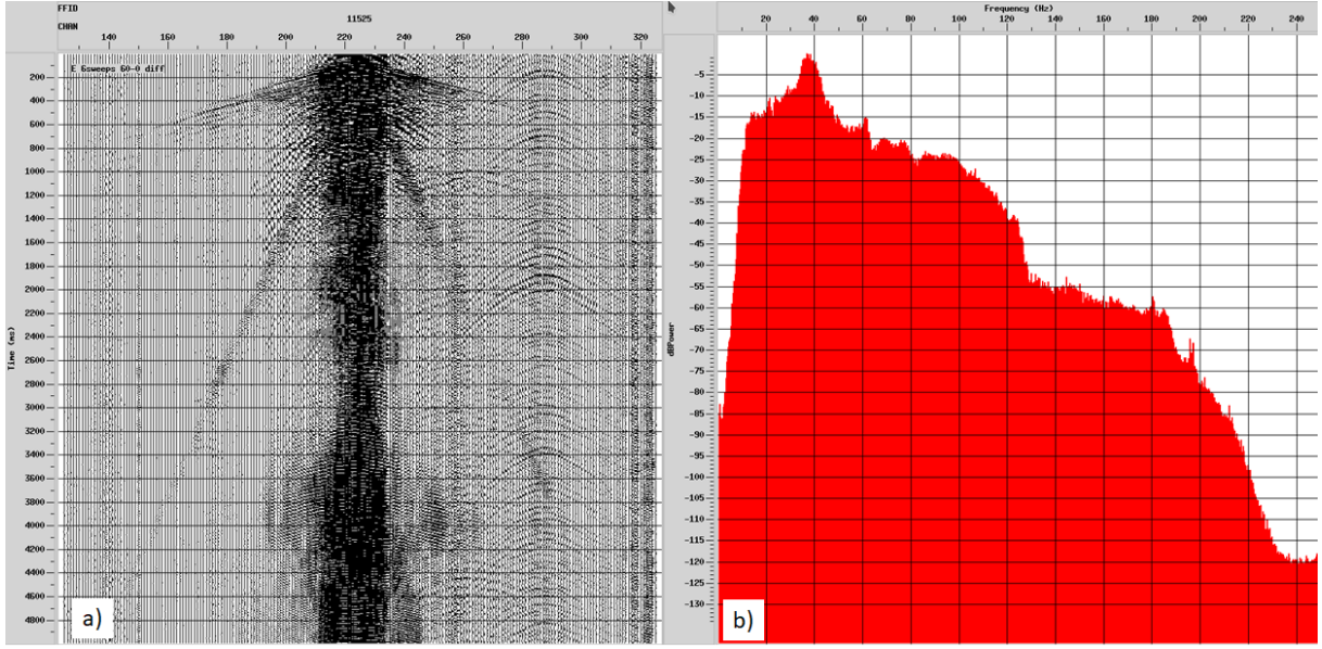
Figure 35. a) Difference between Fig. 33 and Fig. 34, b) The power spectrum of difference
