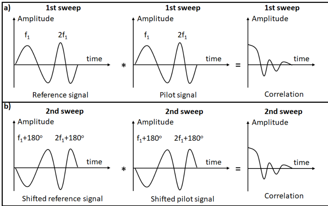
Figure 4. a) Reference signal, a pilot signal of the first sweep without any phase shift, and their correlation, b) Shifted reference signal, shifted pilot signal of the second sweep with a 180 degrees phase shift, and their correlation (revised from Sercel, 1999)
