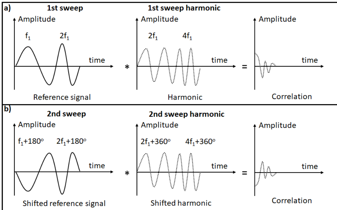
Figure 5. a) Reference signal and harmonic of the first sweep without any phase shift, and their correlation, b) Shifted reference signal, shifted harmonic of the second sweep with a 180 degrees phase shift, and their correlation (revised from Sercel, 1999)
